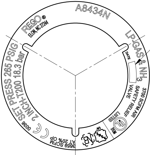
A8434G-32ULN NAMEPLATE REFERENCE COLOR: GREEN
