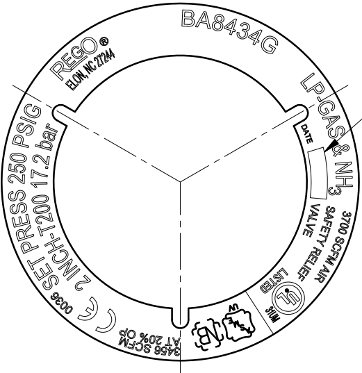
BA8434G-32UL NAMEPLATE REFERENCE COLOR: RED
