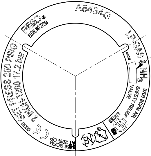
A8434G-32UL NAMEPLATE REFERENCE COLOR: RED
