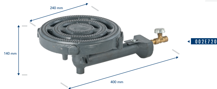
Model 50 LP gas burner
