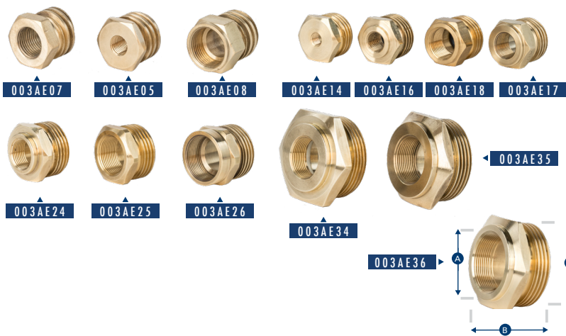
Adapters male ACME X female NPT
